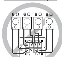
(Speaker terminals)
