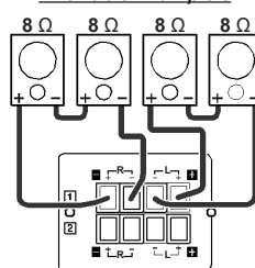
(Speaker terminals)
