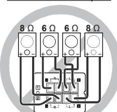
(Speaker terminals)
