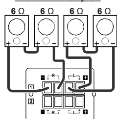
(Speaker terminals)
