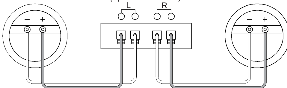
Connected amplifier (Speaker terminals)
